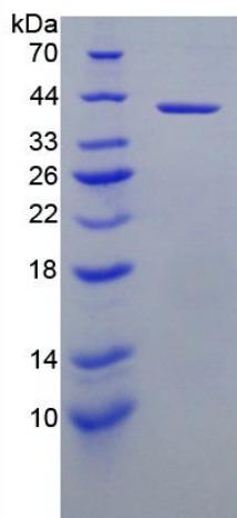
Figure 1. SDS-PAGE
